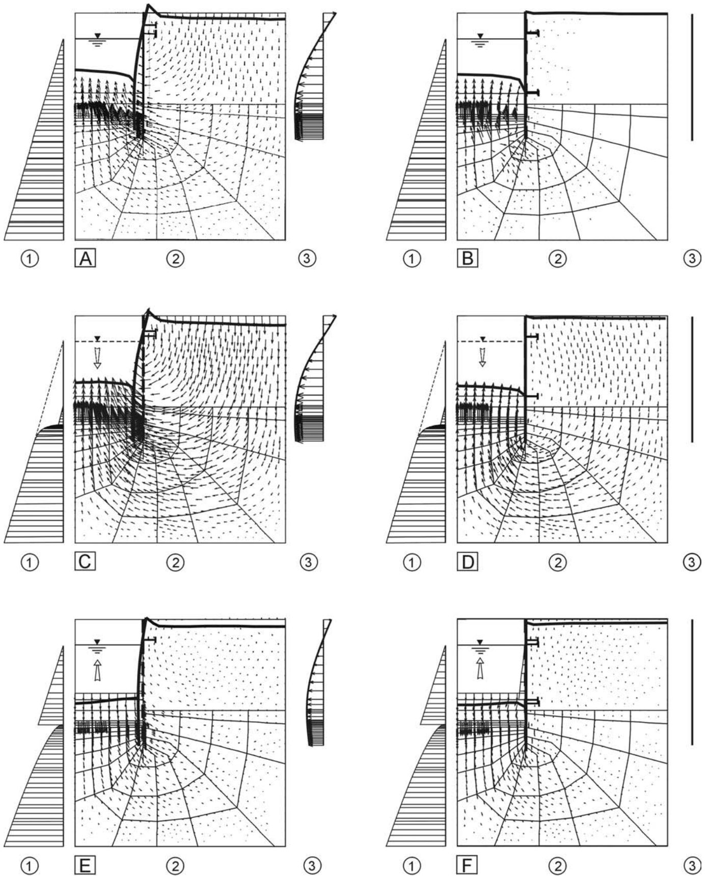
Figure 7 Results of uncoupled simulation for three construction phases, left hand side - deformable retaining wall, right hand side - rigid wall; (A and B) end of excavation under water; (C and D) water level lowering; (E and F) refilling; (1) pore pressure distribution; (2): total displacements and incremental displacement fields; (3) horizontal wall displacements
